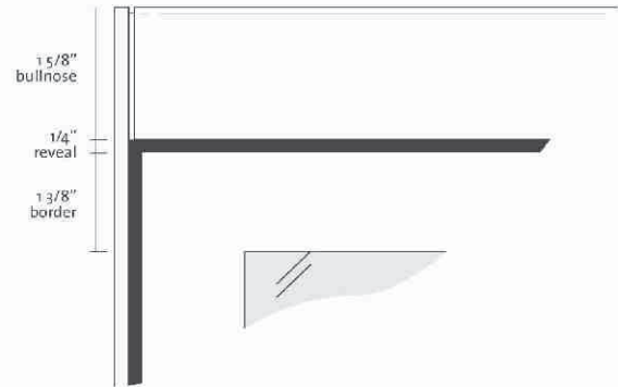
Corner Detail Surface-mounted Bullnose
