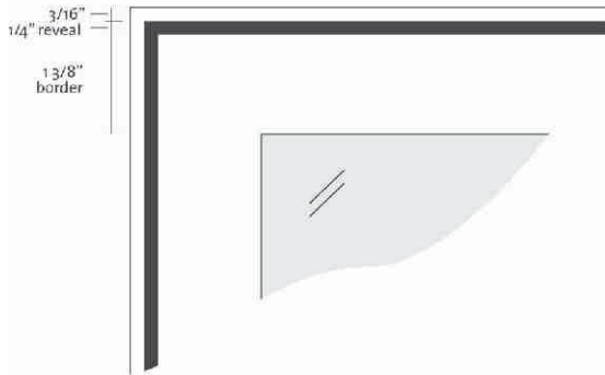
Corner Detail Surface-mounted
